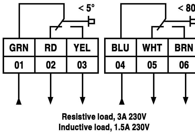
Open/close with integrated auxiliary switch
