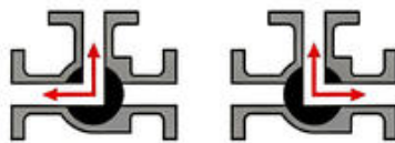
L-type 3-way Ball Valve
