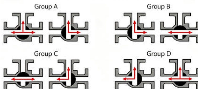
T-type 3-way Ball Valve
