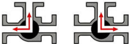
L-type 3-way Ball Valve
