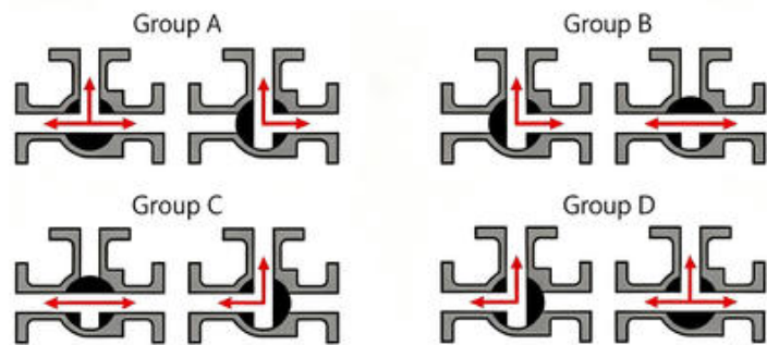
T-type 3-way Ball Valve
